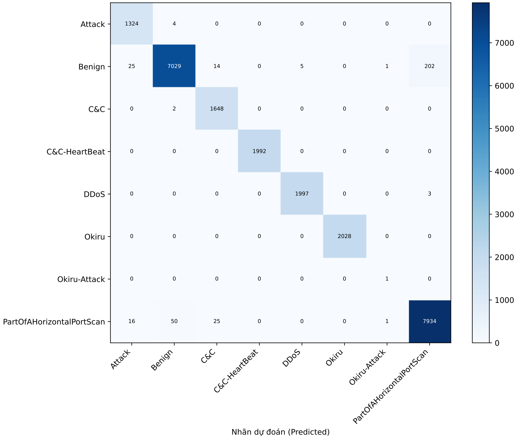
Confusion matrix pooled — counts (seed 42)
