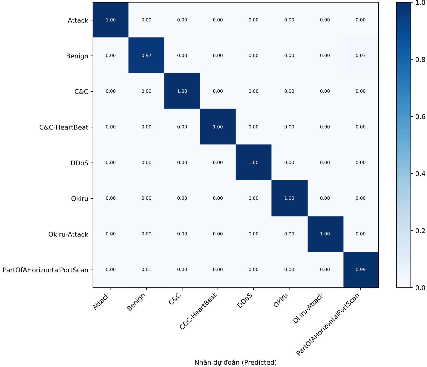
Confusion matrix pooled — normalized by true class (seed 42)
