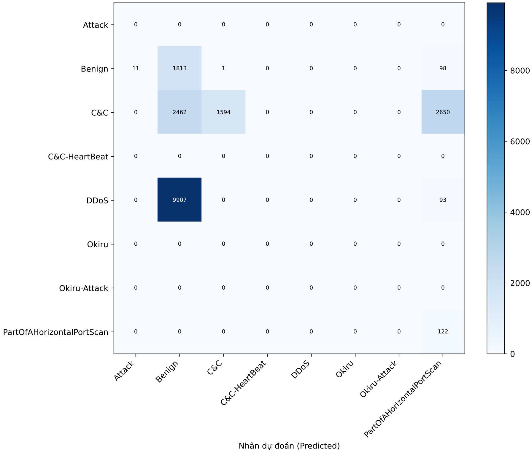
Confusion matrix hardest LOSO 34-1 — counts (seed 42)
