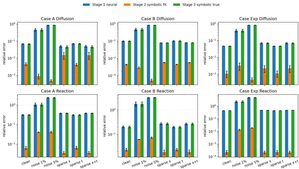
Figure 2: Neural-to-symbolic error propagation. Stage 2 compression error remains small, while Stage 3 true symbolic error tracks the Stage 1 neural true error. This is the empirical signature of bias preservation.
