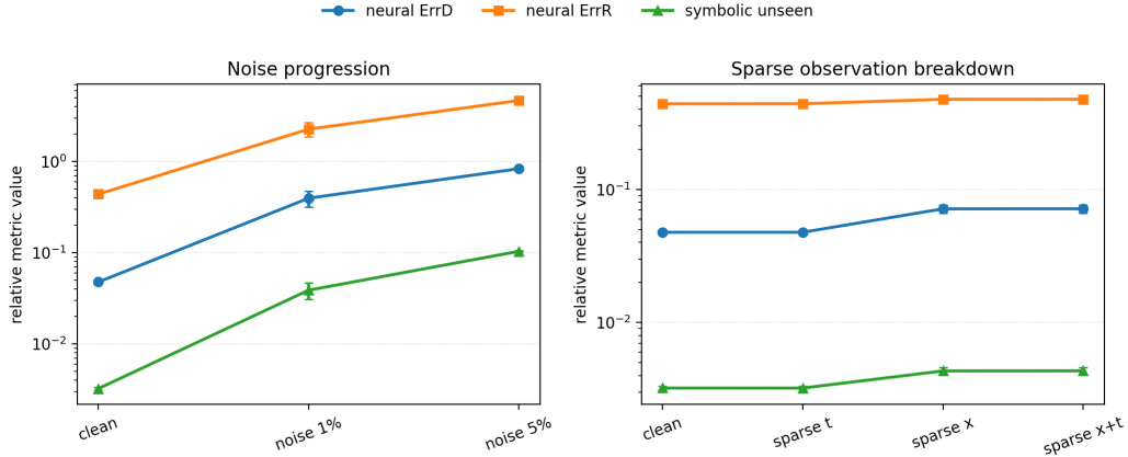
Figure A.3: Case Exp observation-degradation breakdown. Left: neural closure errors and symbolic unseen rollout error deteriorate progressively from clean data to 1% and then 5% noise. Right: temporal stride 2 alone leaves the mismatch benchmark almost unchanged, while spatial stride 2 accounts for nearly all of the sparse-setting degradation.
