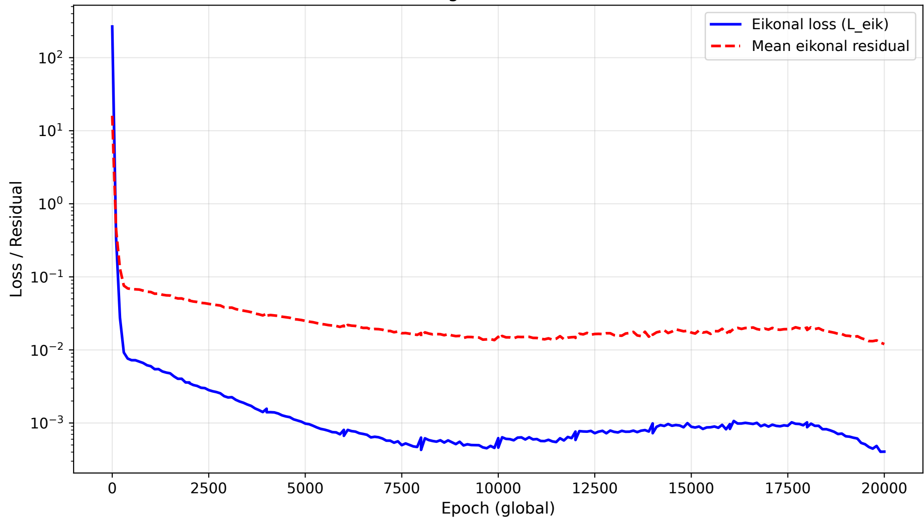
Training Loss & Residual
