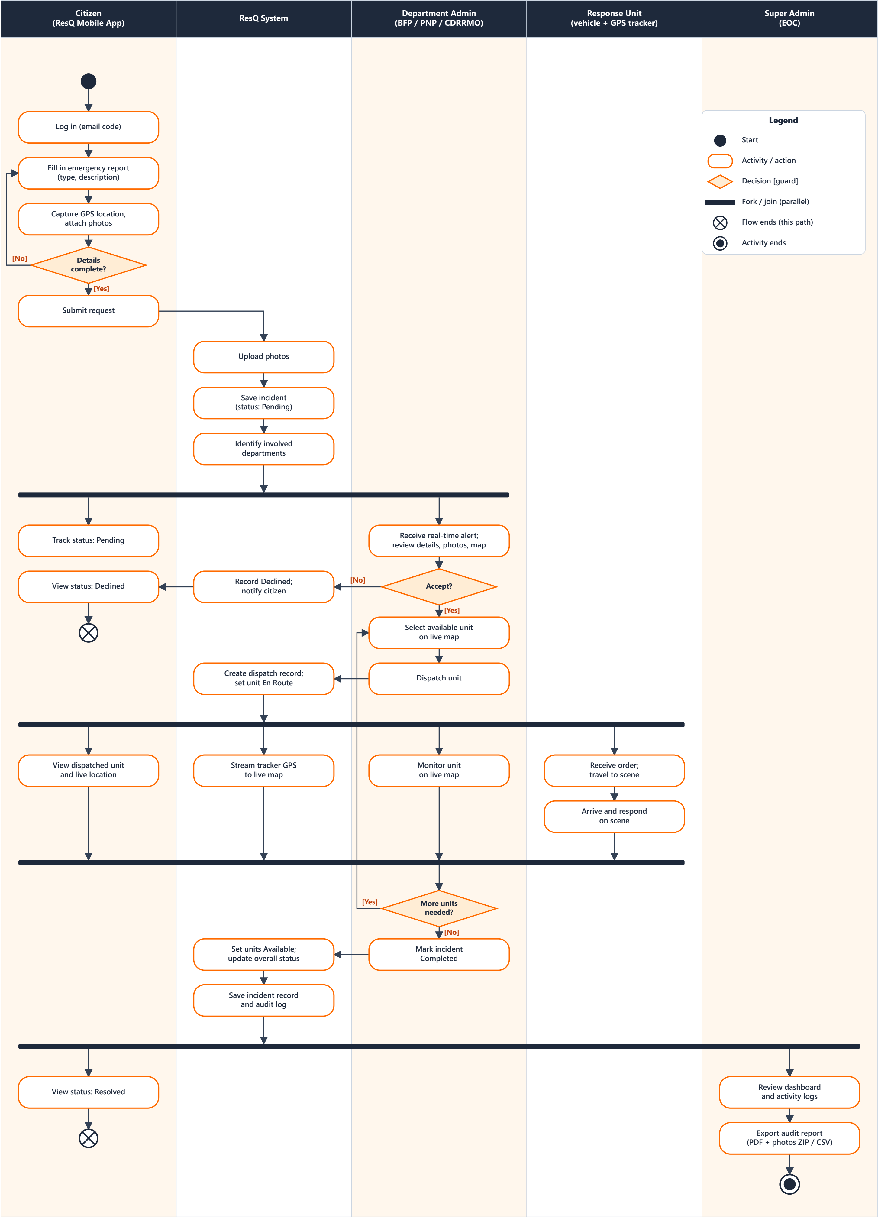
Activity Diagram of ResQ
