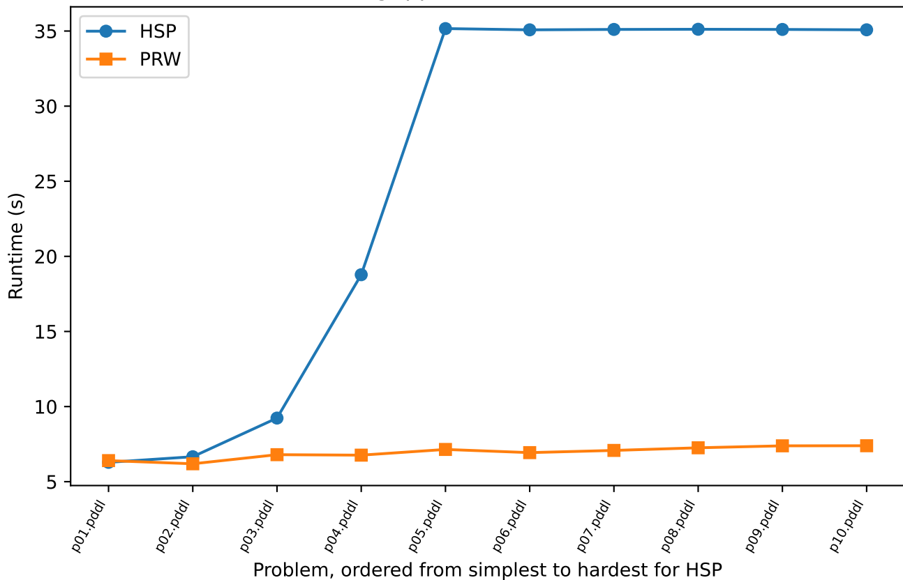
gripper: Runtime (s)
