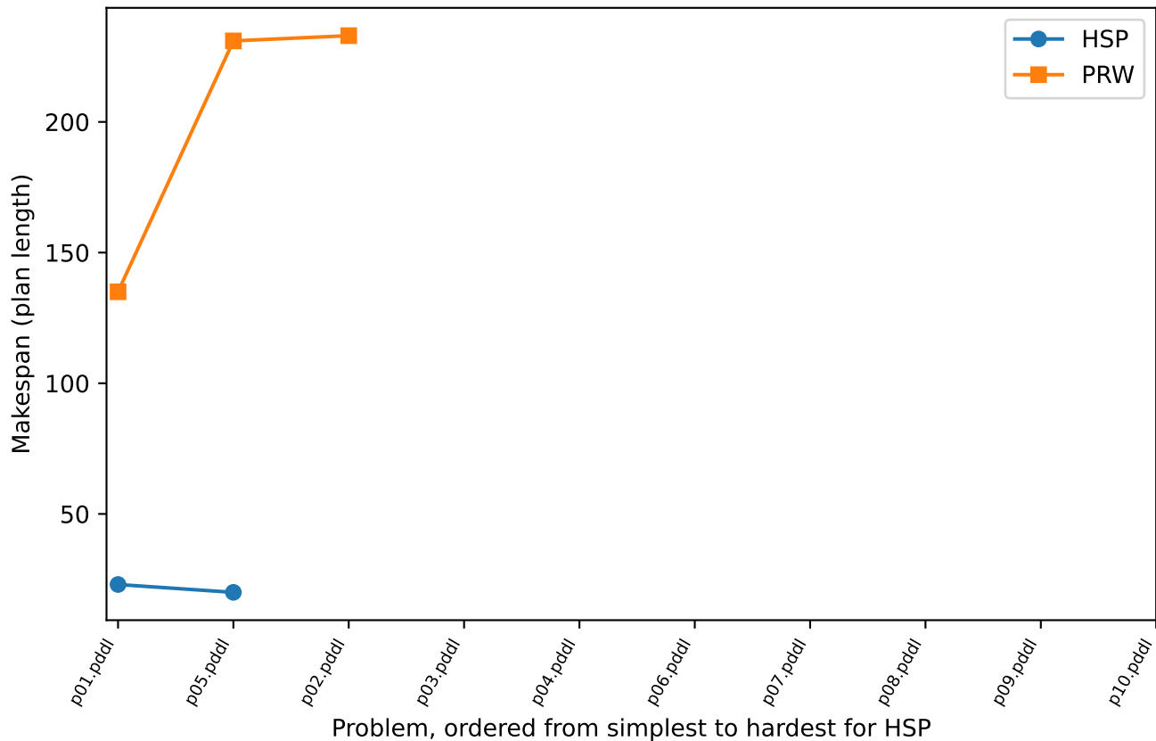
logistics: Makespan (plan length)
