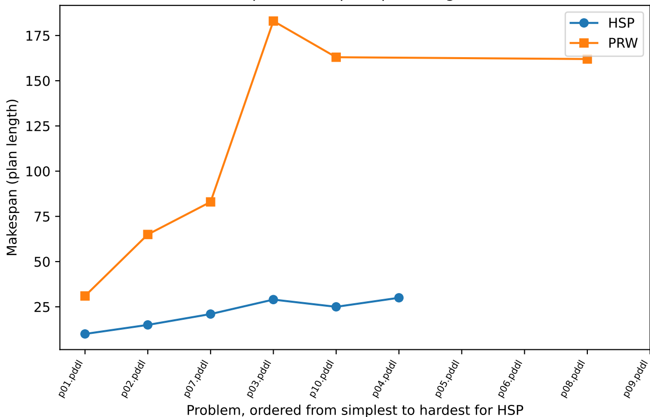
depot: Makespan (plan length)
