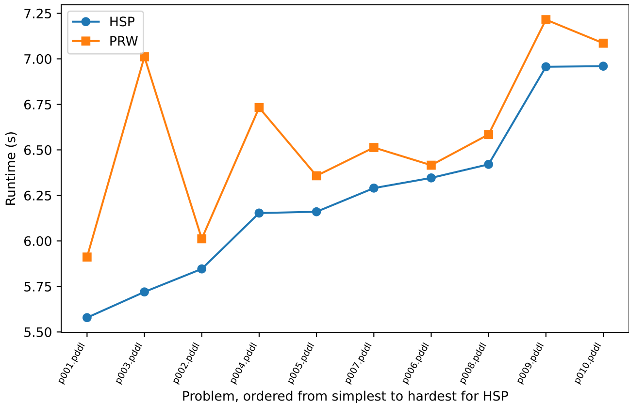
blocksworld: Runtime (s)
