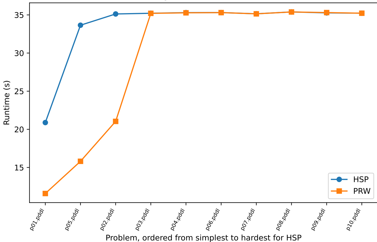
logistics: Runtime (s)
