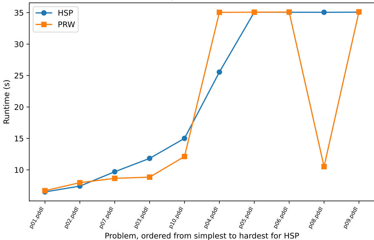
depot: Runtime (s)
