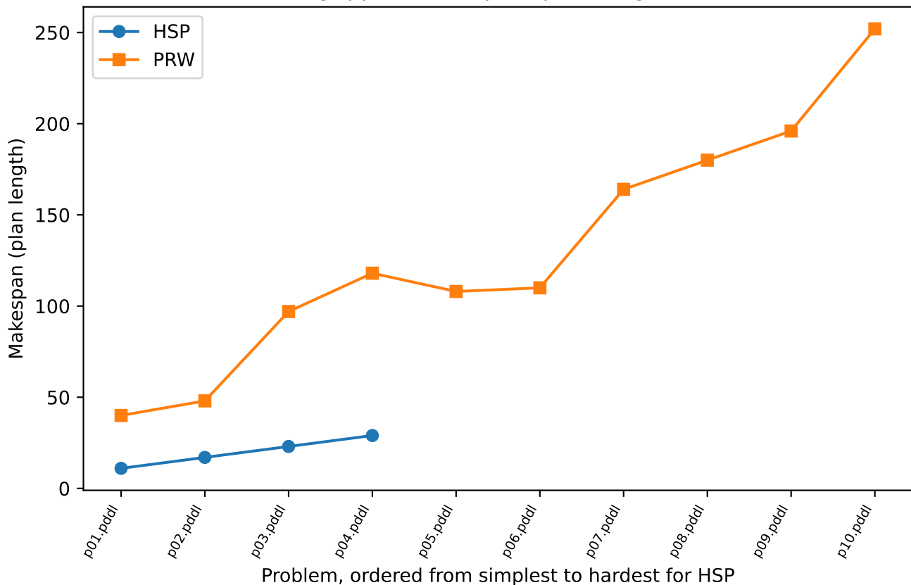
gripper: Makespan (plan length)
