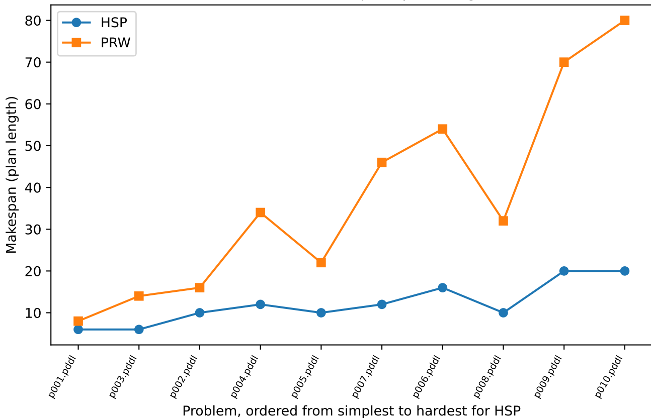
blocksworld: Makespan (plan length)
