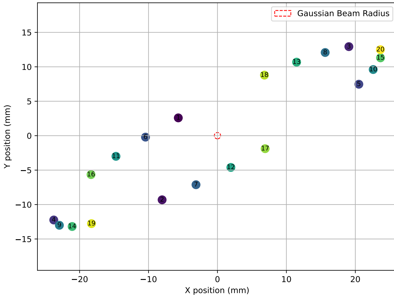
Multi-Pass Cell Spot Distribution with Eigenmode Overlay ( R=300 mm, L=550 mm, n=20 )
