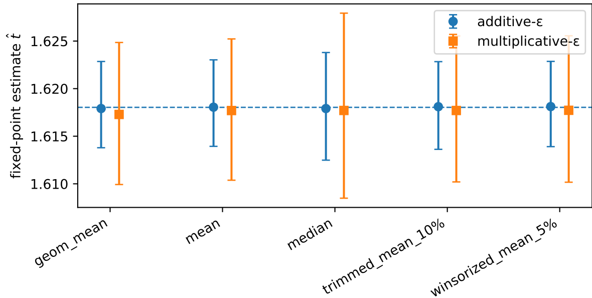
Aggregator estimates: median \pm 95% CI
