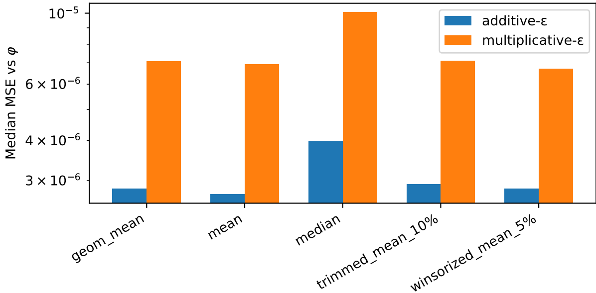
Median MSE to \varphi by estimator and model (lower is better)
