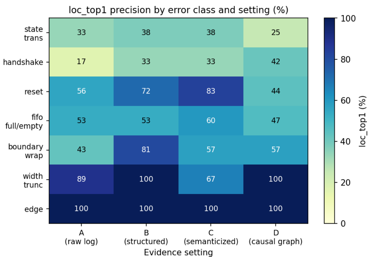
Figure 3: Error-class x setting heatmap
