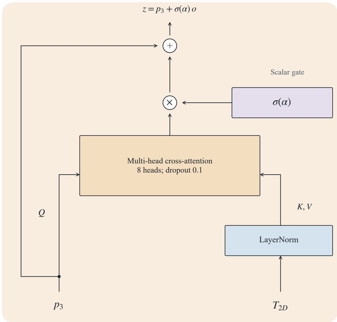
(b) CrossGate module
