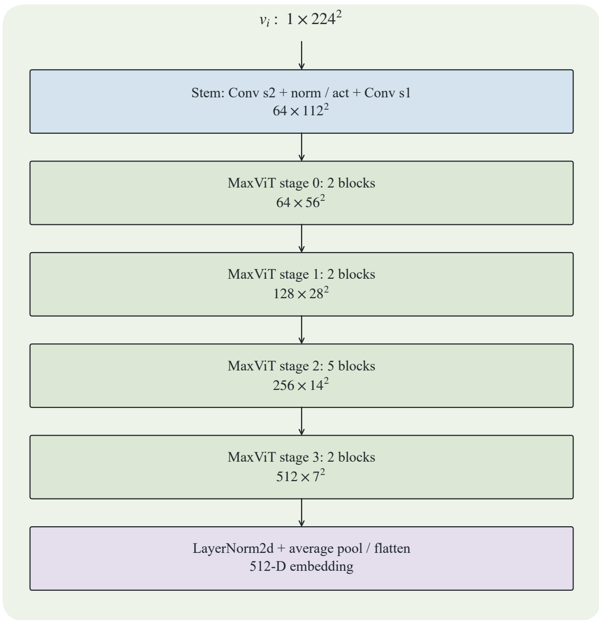
(c) MaxViT-Tiny encoder (each view)
