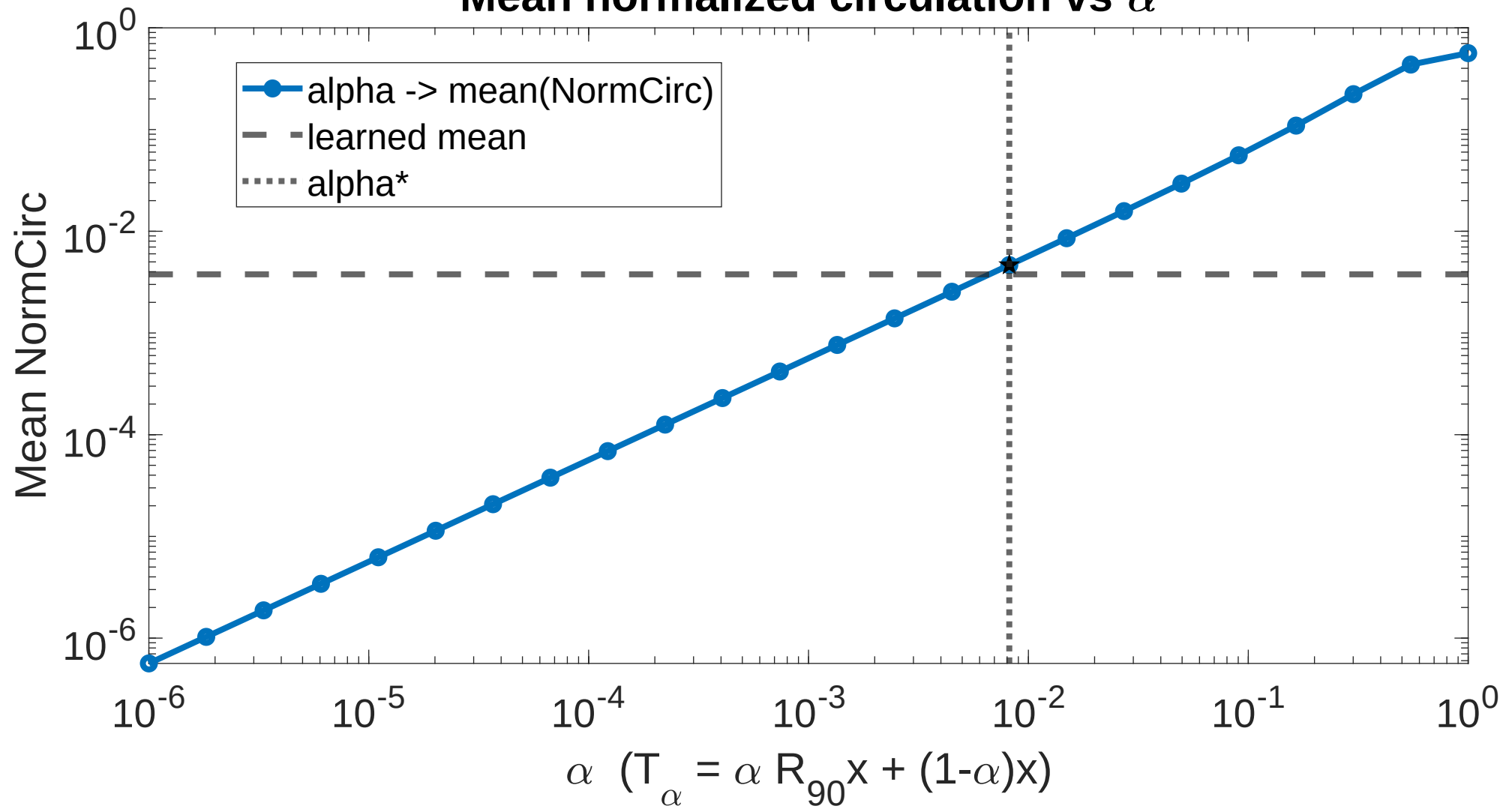
Mean normalized circulation vs \alpha
