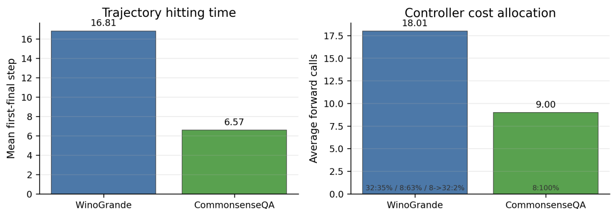
Expanded trajectory analysis (500 samples per task, stride=1)
