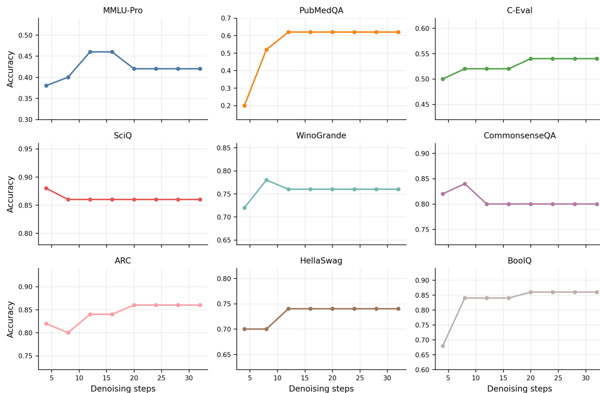
Accuracy vs diffusion steps (9 tasks, 50 samples each)
