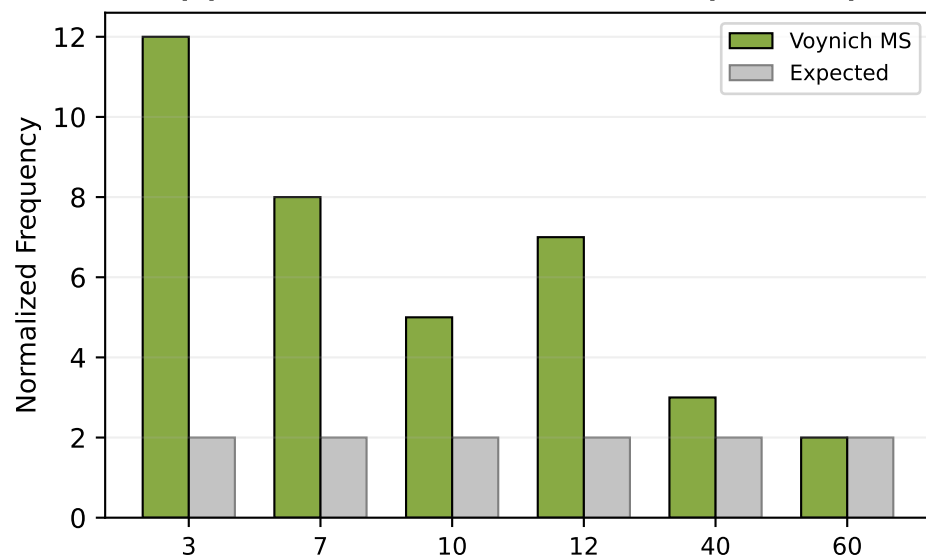
(c) Sacred Number Distribution (INV-027)
