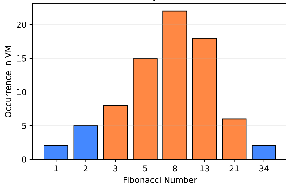
(c) Sacred Number Distribution (INV-027)
