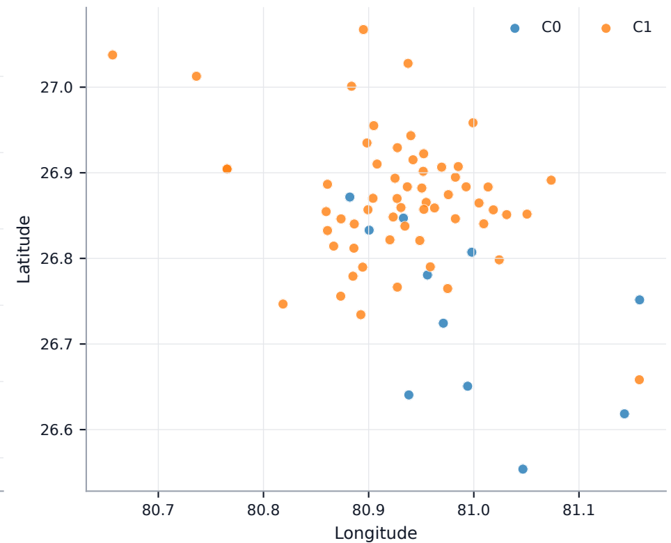
Lucknow: sensor clusters (k=2)
