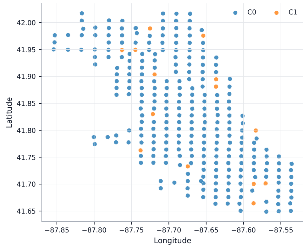
Chicago: sensor clusters (k=2)
