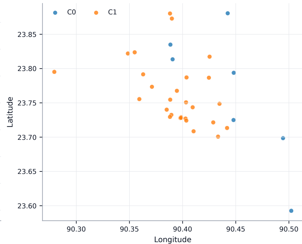
Dhaka: sensor clusters (k=2)
