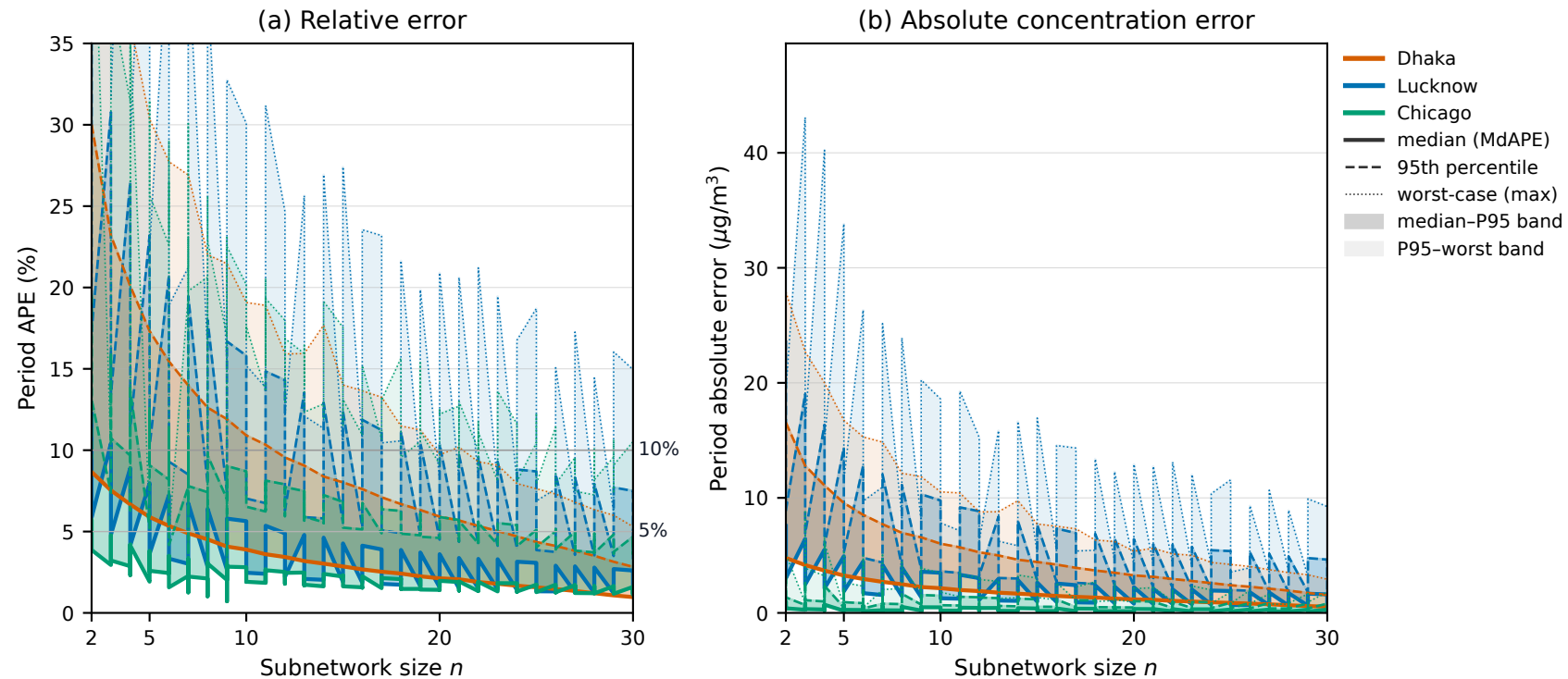
Period subnetwork error — median, 95th percentile, and worst observed draw across B = 10,000 SRSWOR Monte Carlo subnetworks
