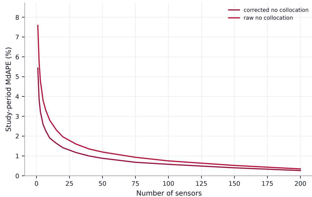
Raw vs corrected, collocations excluded
