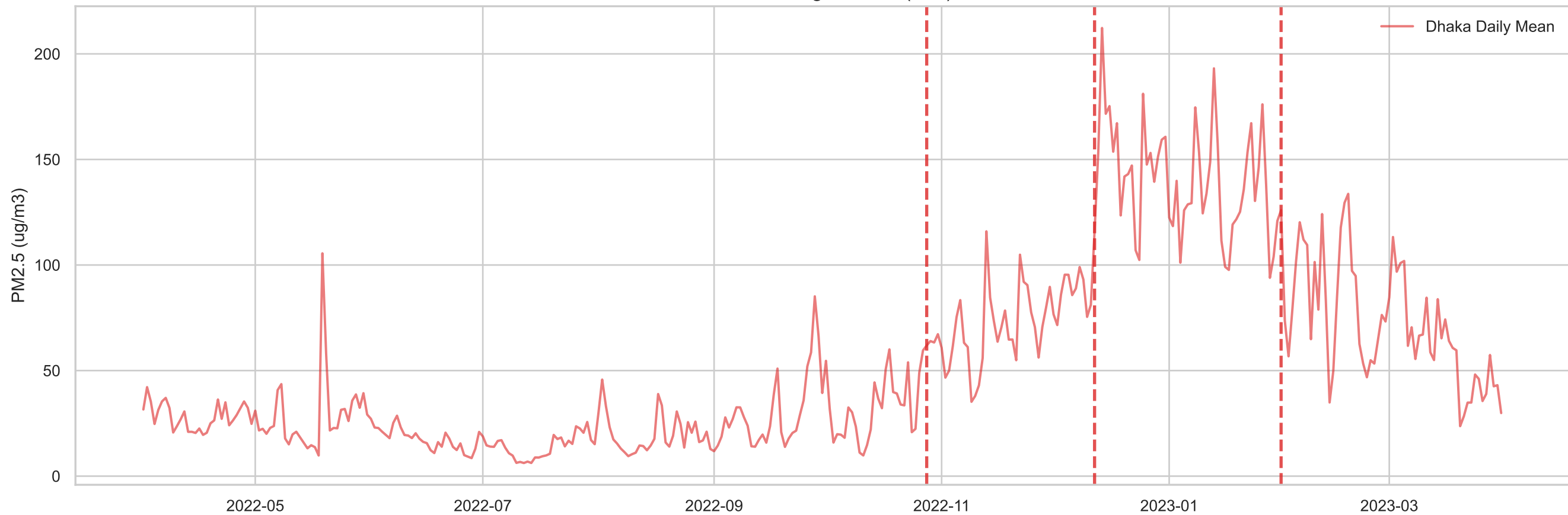
Dhaka: Change-Points (n=3)
