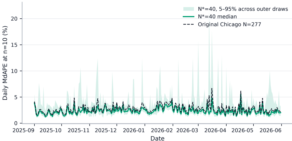
Daily Chicago MdAPE under N^*=40 finite-population draws
