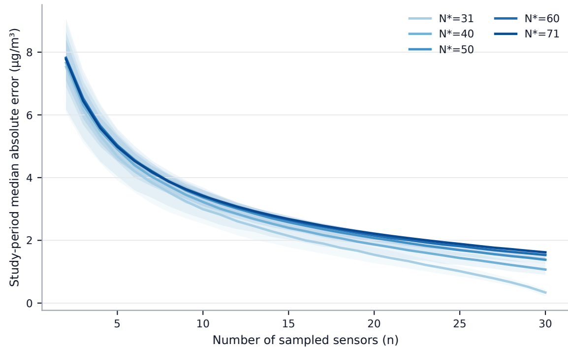
Phase 3 absolute-error sensitivity
