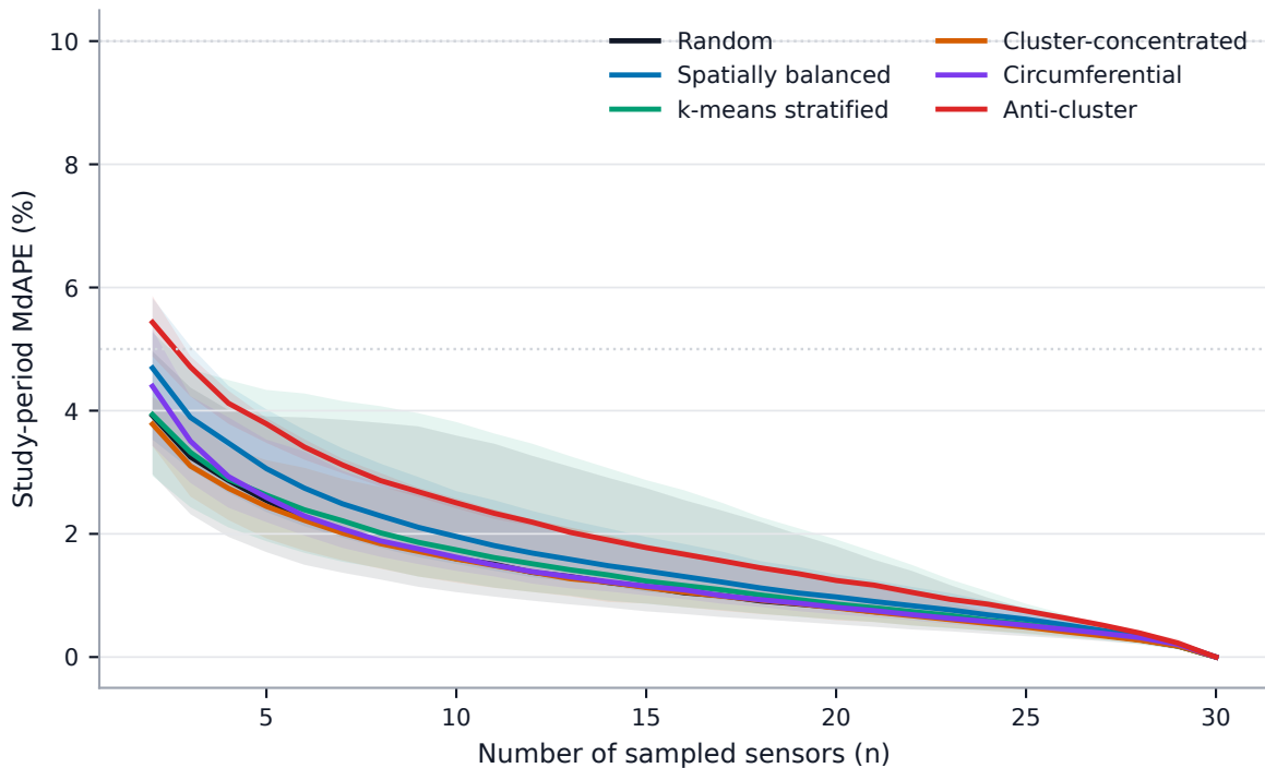
Chicago selection strategies at N^*=30
