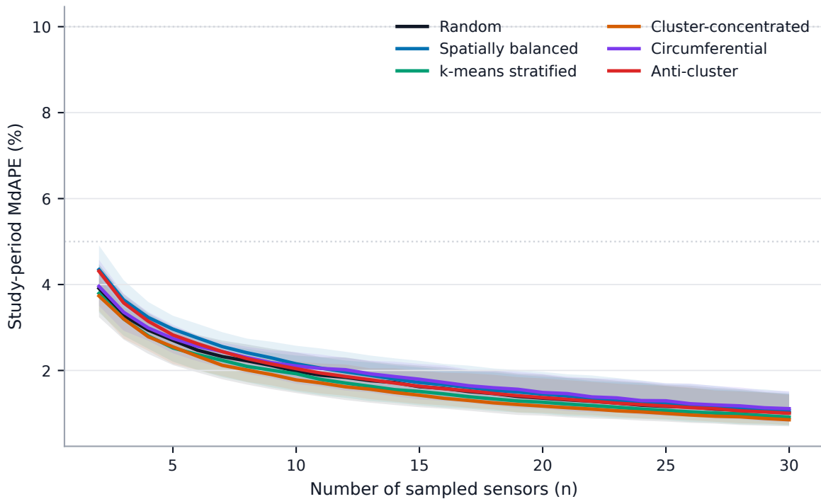
Chicago selection strategies at N^*=70
