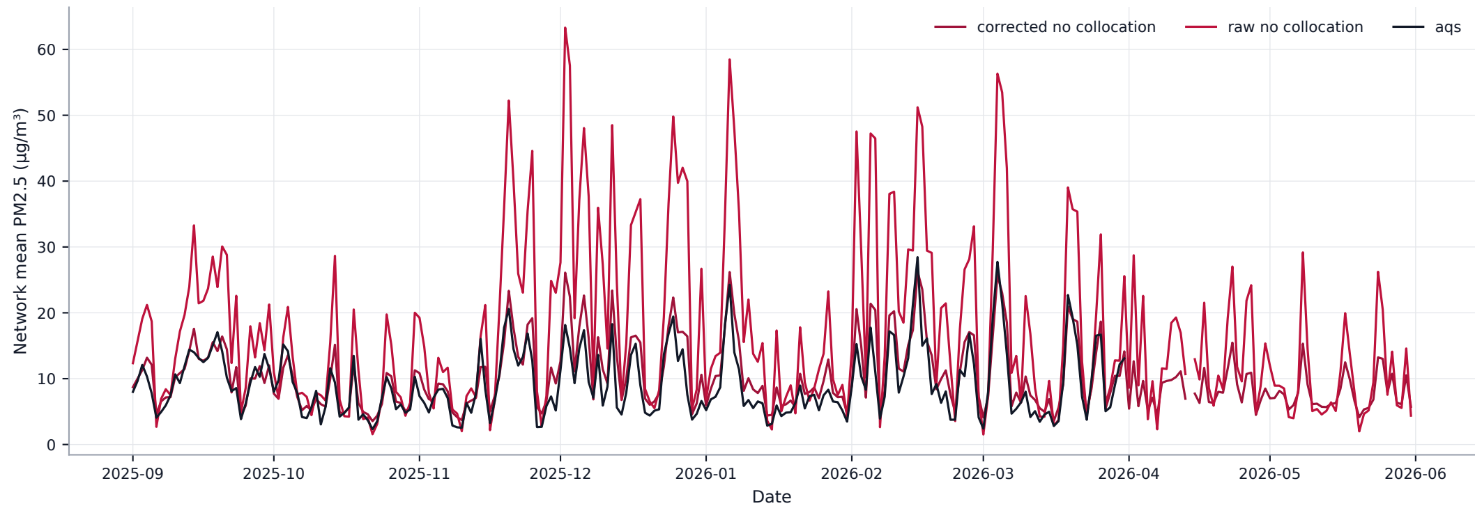
S03. Chicago daily network mean: corrected LCS, raw LCS, and AQS context
