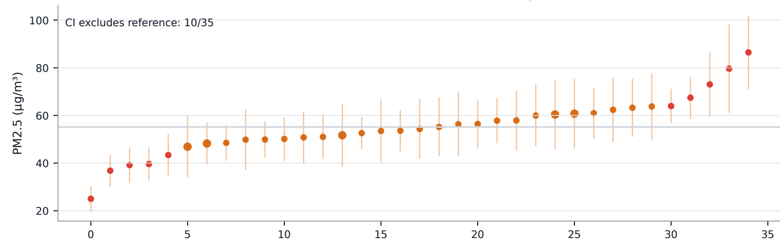
Lucknow: source-resolution AR(1) stationarity screen
