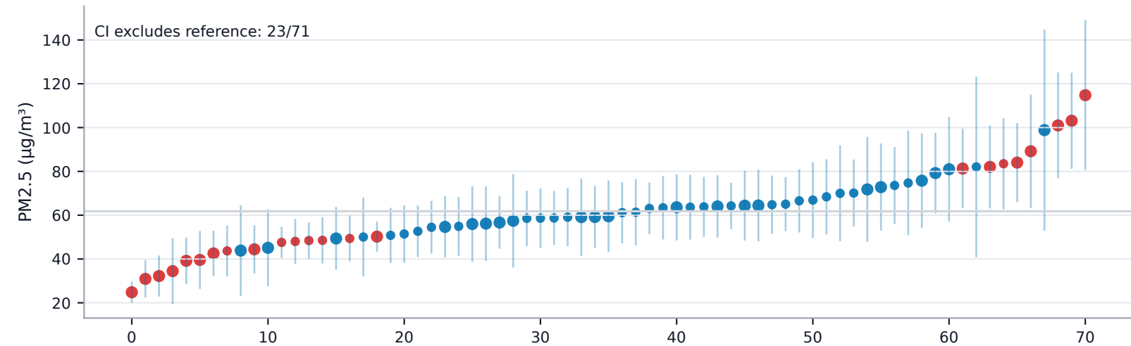
Chicago: source-resolution AR(1) stationarity screen
