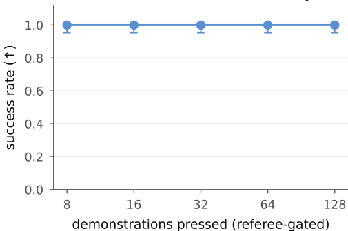
Lift, demonstration count at the study truth
