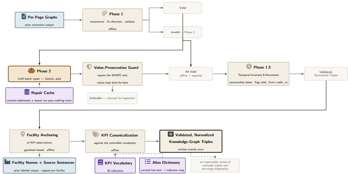
Figure 11: Validate & Normalize, detailed — internal structure of the Validate & Normalize block in Figure 9.
