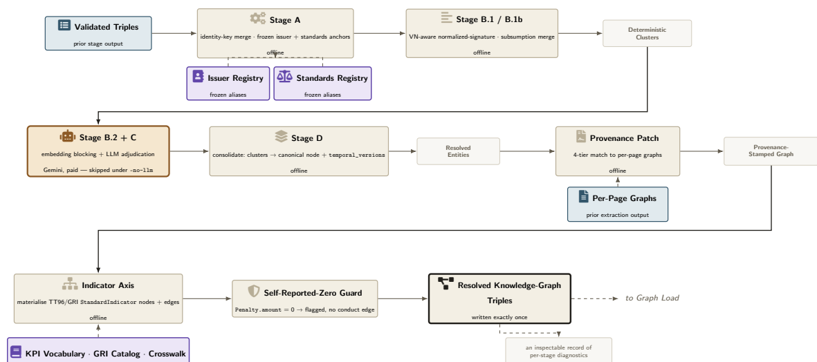
Figure 12: Entity Resolution & Indicator Axis, detailed — internal structure of the Entity Resolution & Indicator Axis block in Figure 9.
