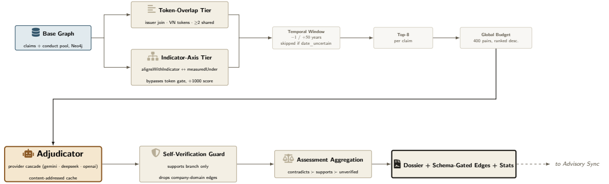
Figure 14: Claim–Conduct Cross-Check, detailed — internal structure of the Claim–Conduct Cross-Check block in Figure 9.
