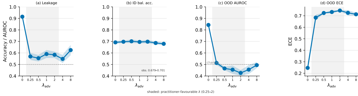
Figure 1: The intervention, four views, one axis. Leakage falls to its chance floor and in-distribution balanced accuracy does not degrade — both favourable. Over the same range OOD AUROC collapses through chance and inverts, and out-of-domain calibration error triples. A developer monitoring the first two panels would see nothing wrong.
