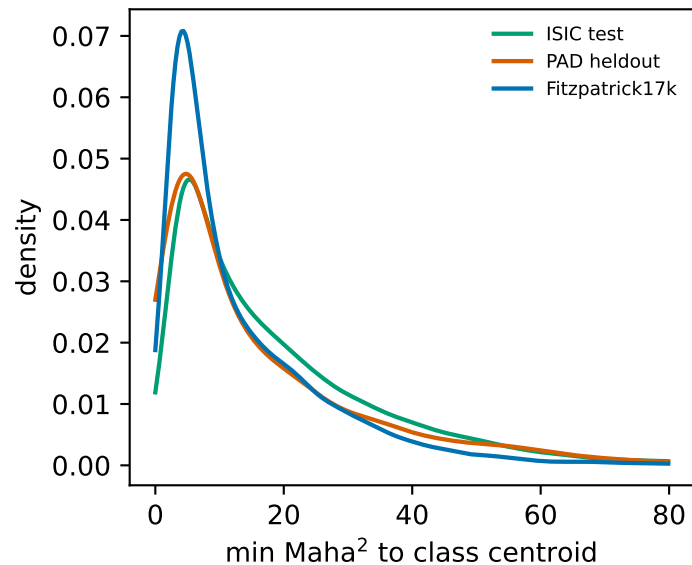
\lambda_{\text{adv}} = 2
