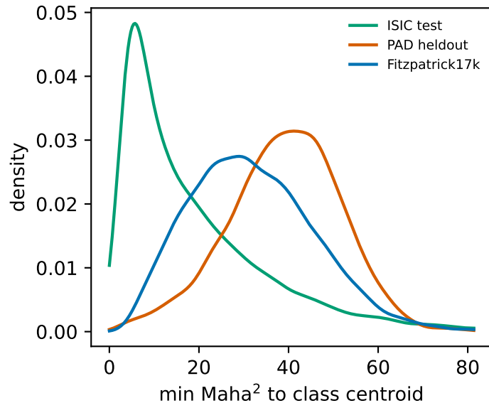
\lambda_{\text{adv}} = 0
