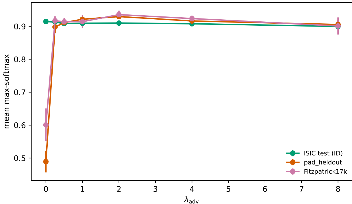
13.3: confidence on unseen domains
