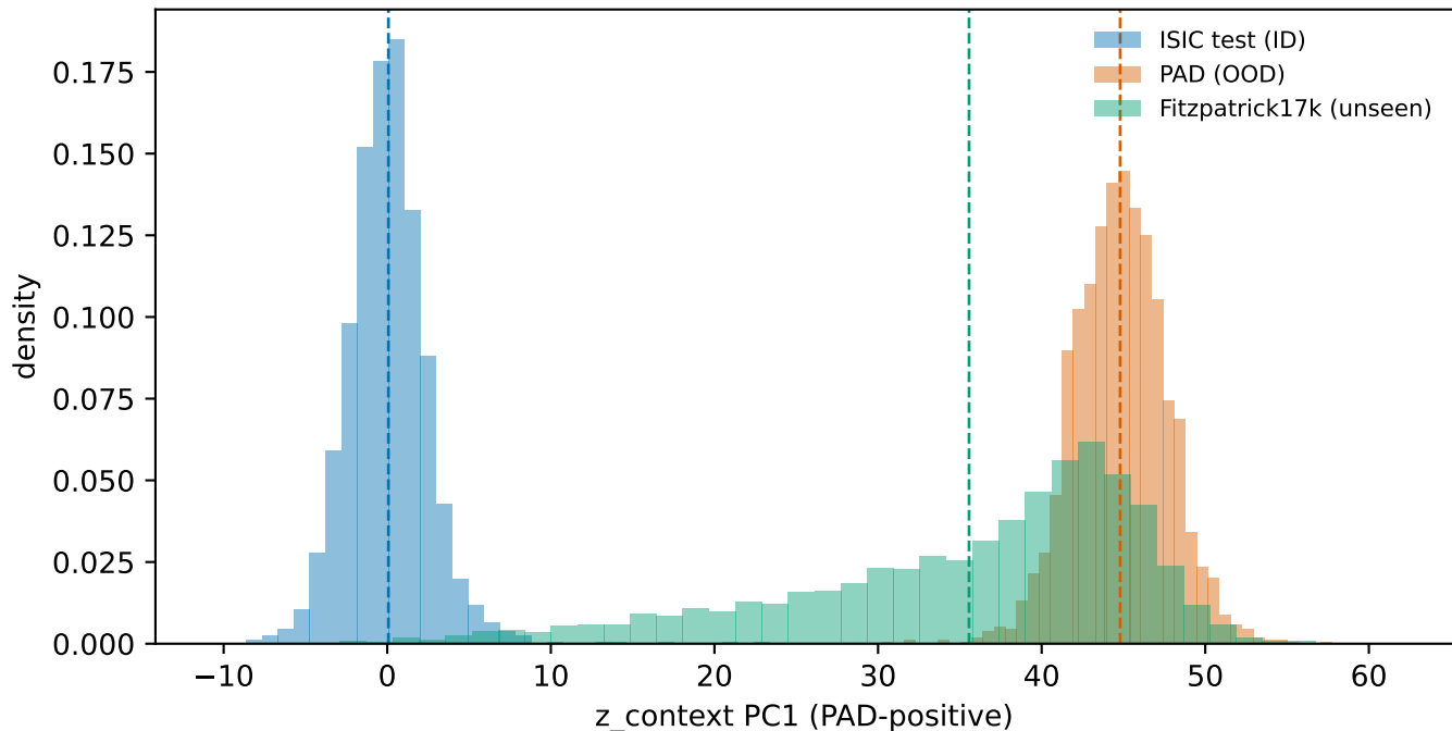
Unseen-domain projection on the 1-D context axis (eval only; Fitzpatrick17k images not redistributed)
