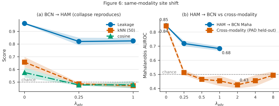
Figure 6: A same-modality site shift separates the two claims. (a) Barcelona to HAM10000: leakage falls and the detectors with headroom cross chance. (b) With the roles reversed to restore headroom, Mahalanobis falls from a baseline matching the cross-modality sweep but stops above chance, while the cross-modality sweep continues below it.
