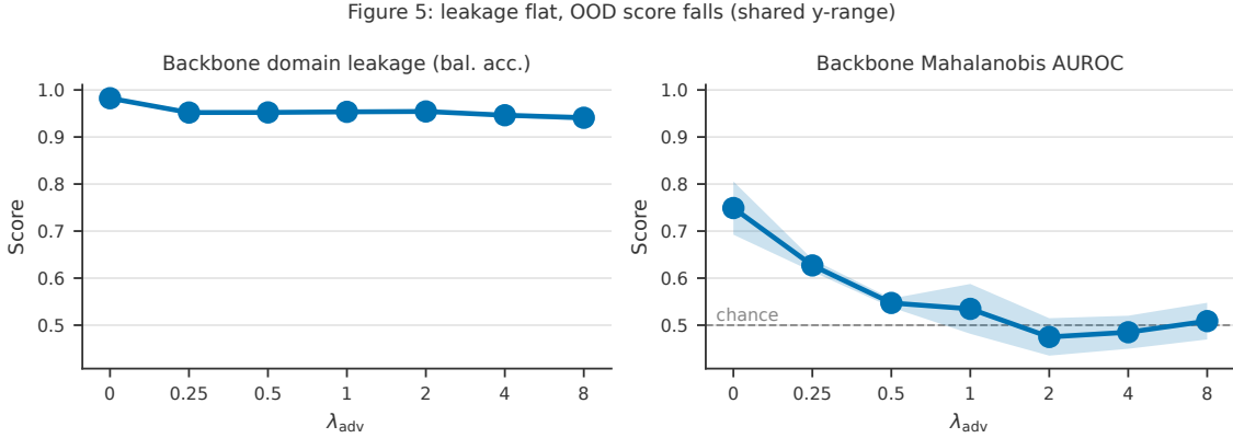
Figure 5: Leakage does not mediate the collapse. At the pre-projection backbone the domain probe stays flat across the sweep while Mahalanobis AUROC falls. Domain information remains linearly decodable and detection degrades regardless.
