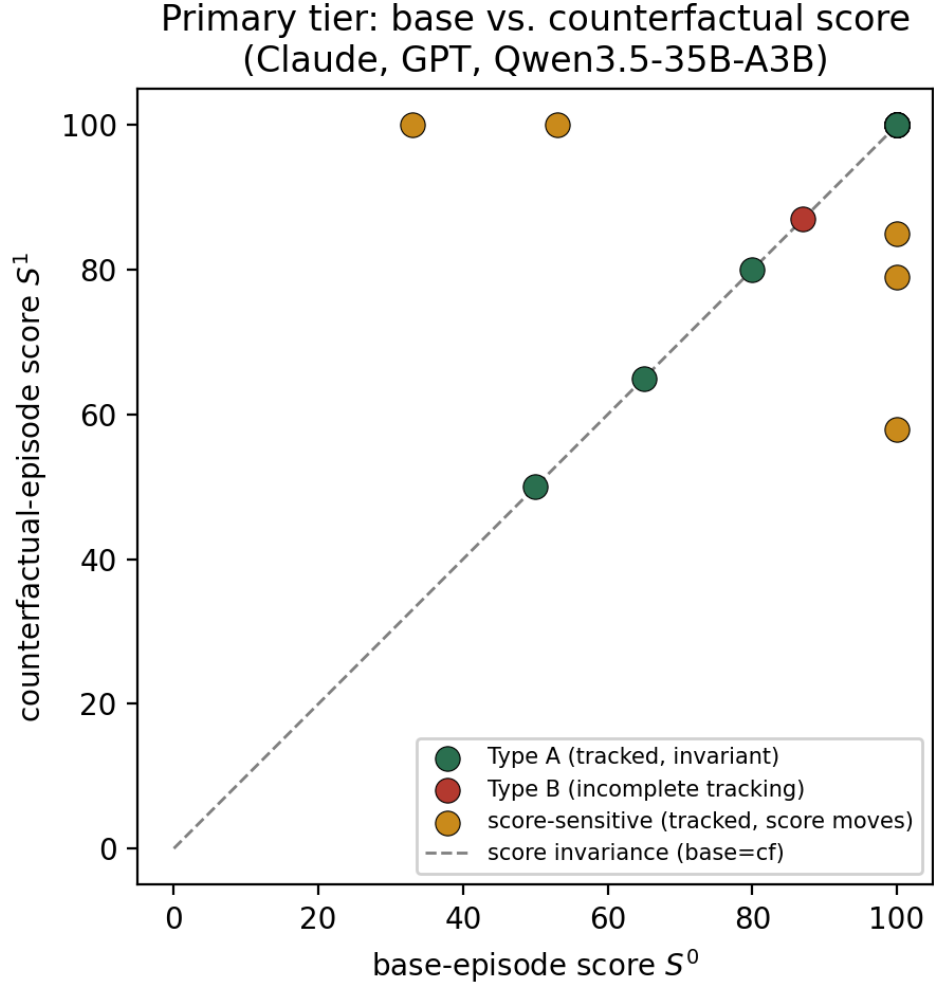
Figure 2: Study 1 primary lanes: paired base vs. counterfactual scores on valid pairs. Ablation and exploratory lanes are not pooled into Table 7.
