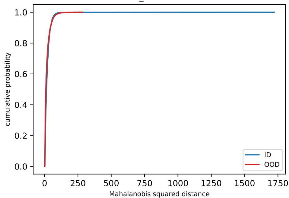
runB_orth1 -- ECDF
