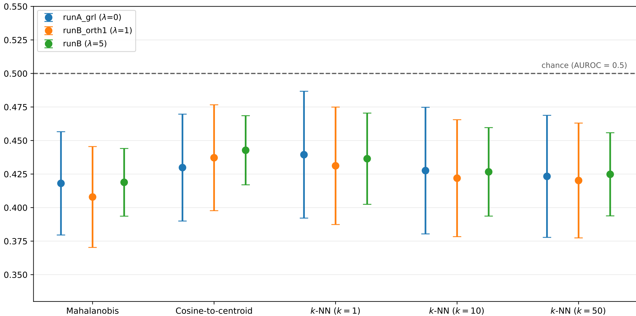
directed OOD AUROC (ISIC-test vs. PAD-UFES)
