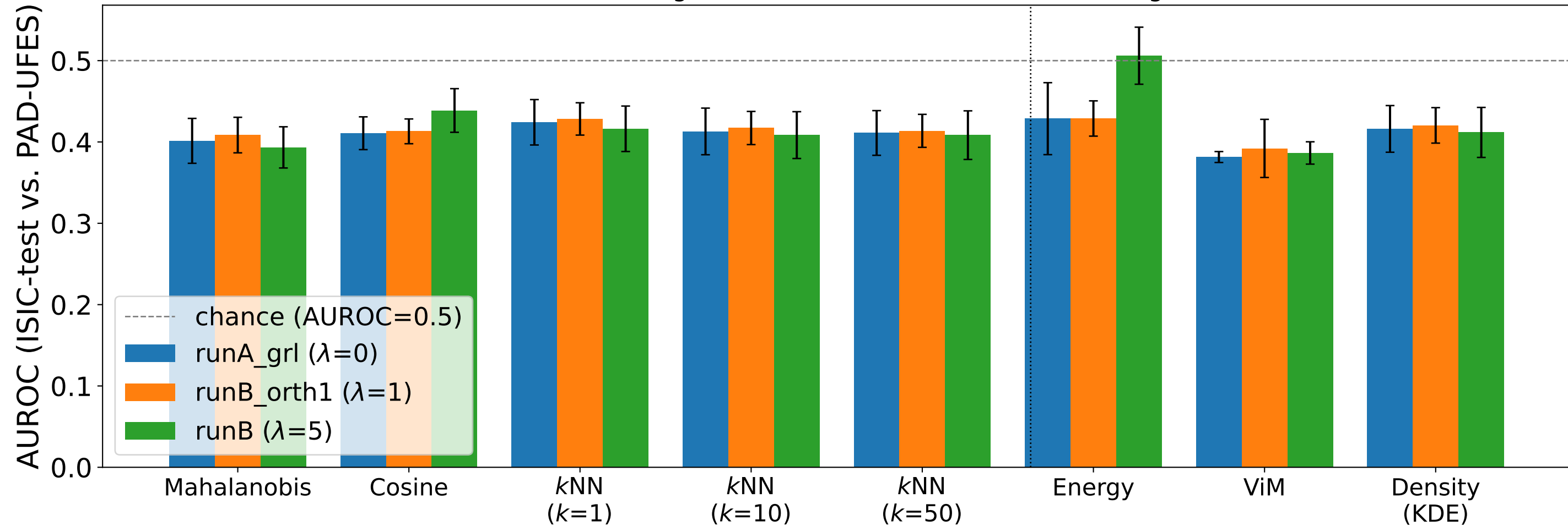
E2.6/E2.8 -- eight scorers on the identical embeddings
