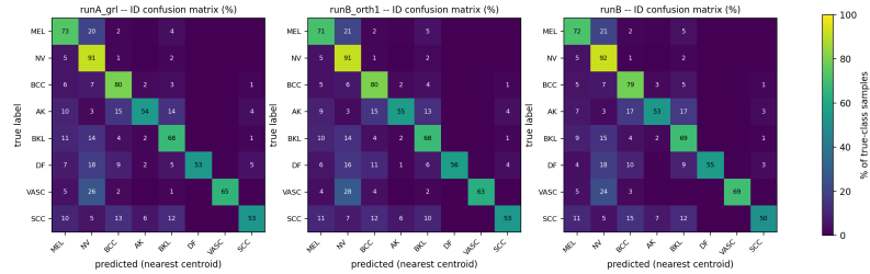
Figure S5: Full ISIC-test nearest-centroid confusion matrix, all 8 classes.
