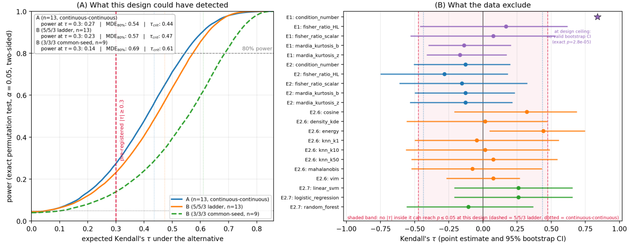
Figure S8: (A) Power of each exact permutation design against expected \tau ( 2 \times 10^4 simulated datasets per point, common random numbers; \alpha = 0.05 , two-sided). Dotted vertical lines mark each design's \tau_{crit} ; the dashed red line marks the pre-specified |\tau| \geq 0.3 criterion, which falls below every \tau_{crit} . (B) Observed \tau and 95% BCa bootstrap intervals for all 21 reported associations. The shaded band spans \pm \tau_{crit} for the 5/5/3 ladder: no |\tau| inside it can reach p \leq 0.05 at this design. Condition number vs. \lambda_{orth} sits at the design ceiling and is shown as a point without an interval (see Table S9).
