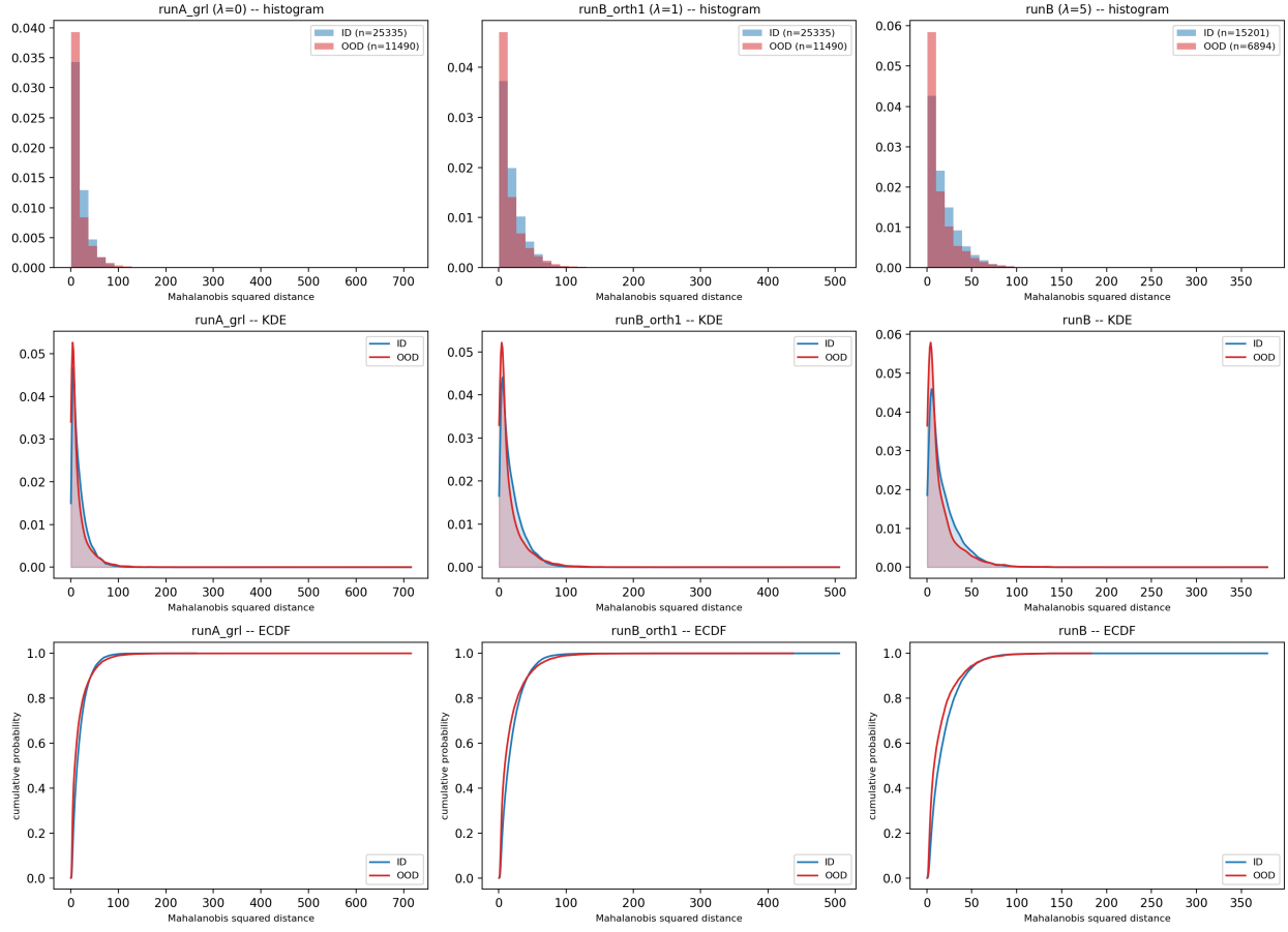
Figure S4: ID vs. OOD Mahalanobis squared-distance distributions, all three rungs.
