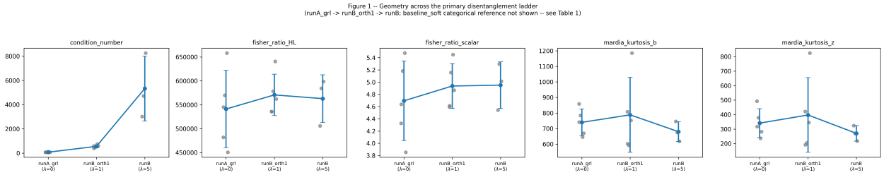
Figure S1: All five geometry metrics across the disentanglement ladder.
