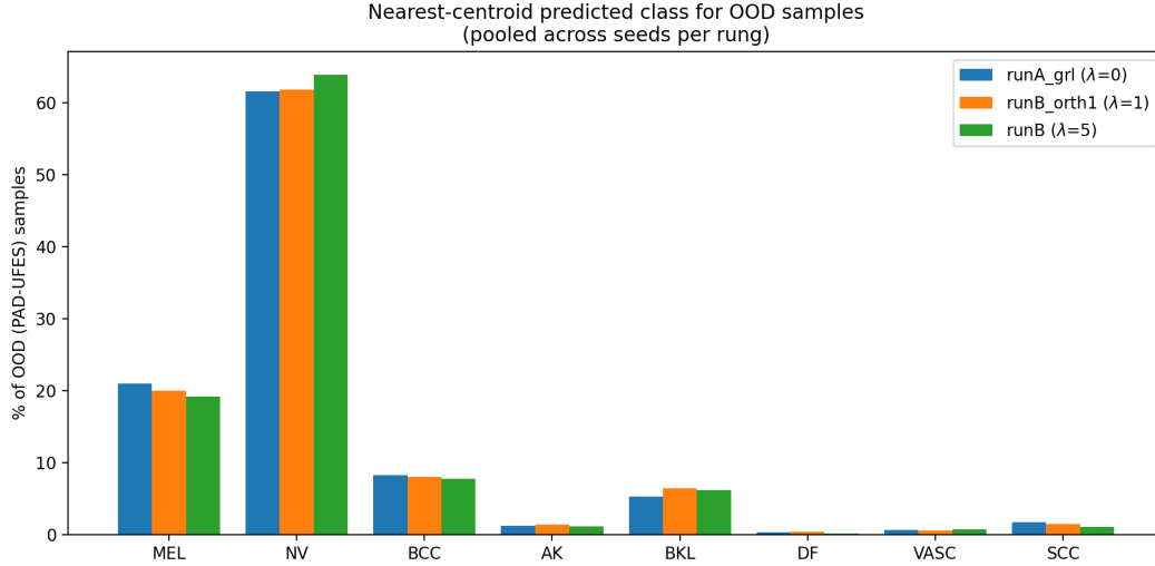
Figure S6: Full PAD-UFES nearest-centroid predicted-class distribution, all 8 classes.
