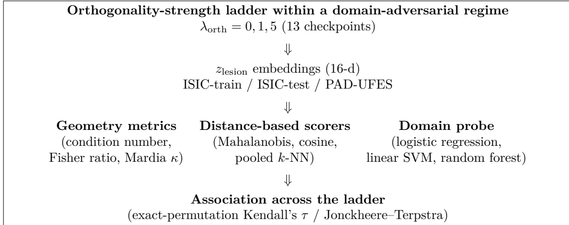
Figure 1: Study design. An orthogonality-strength ladder within a domain-adversarial regime comprises three checkpoint families ( \lambda_{\text{orth}} = 0, 1, 5 ) sharing architecture and representation dimensionality. It is used to test whether an implicit assumption—that representation geometry reflects reliability-estimation quality—holds across changes in orthogonality strength within that regime. Geometry metrics, three distance-based scorers, and domain-information probes are computed on identical embeddings for each of 13 checkpoints (Section 3.1).
