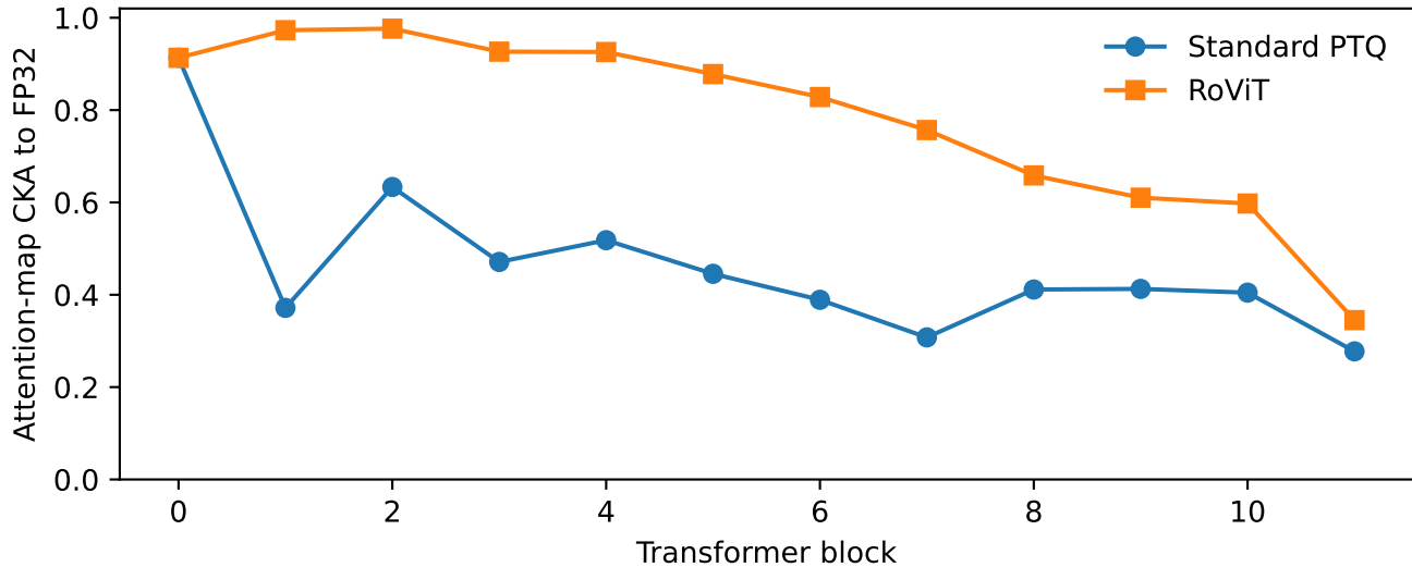
Attention topology preservation (W4A4)
