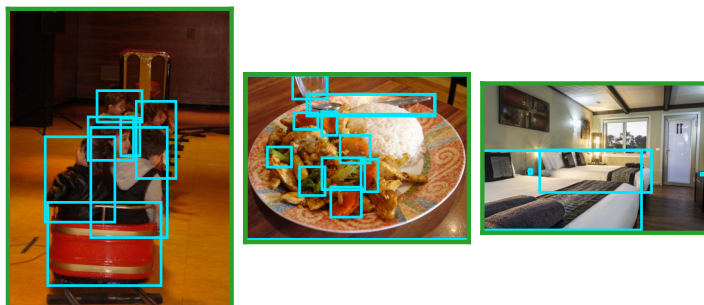
MS COCO 2017
