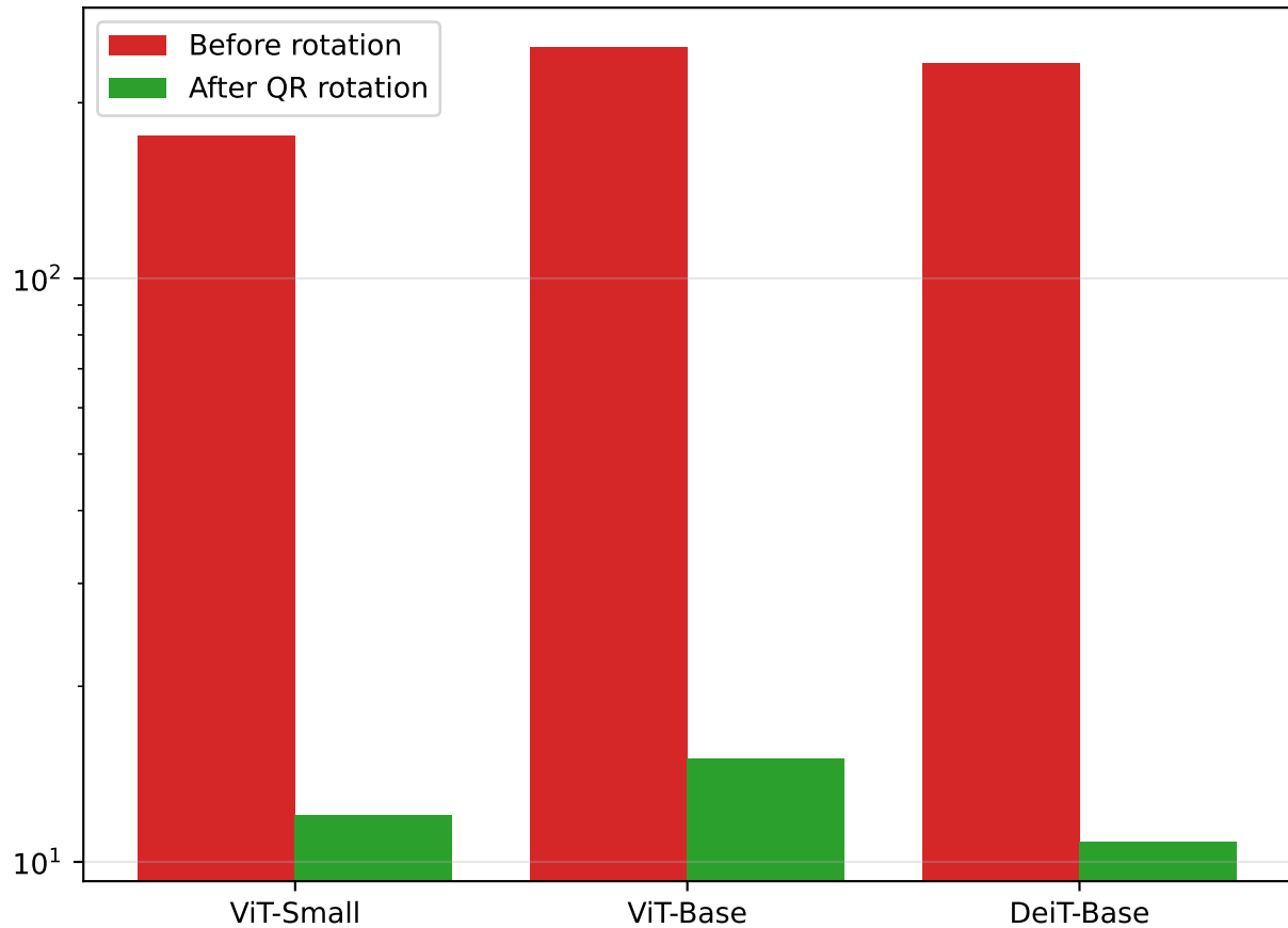
Average M/ \mu ratio (post-GELU MLP layers)
