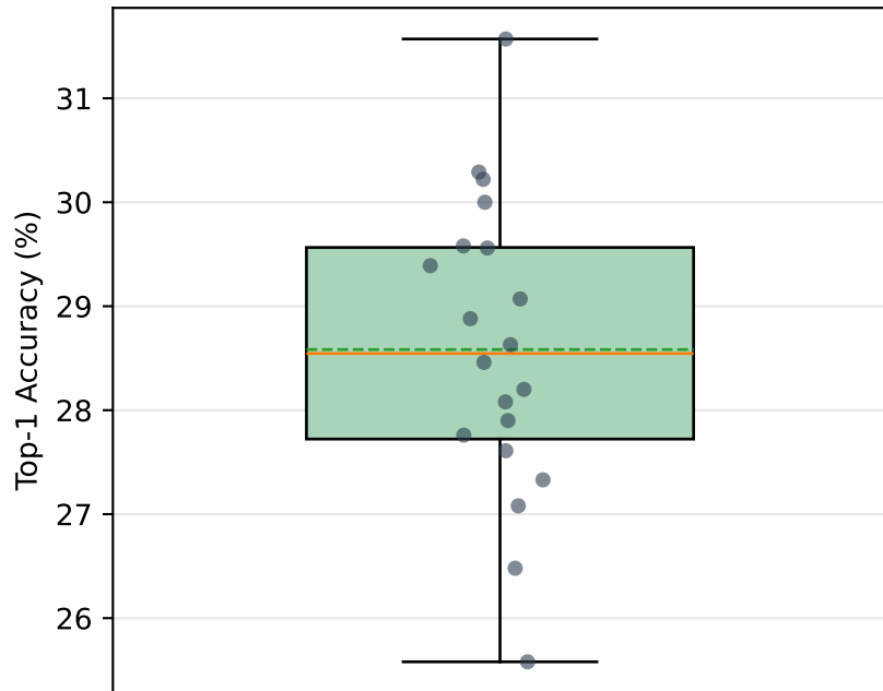
RoViT ViT-Base W4A4 mean 28.58 \pm 1.437 (n=20)
