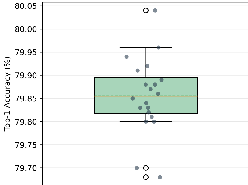
RoViT ViT-Base W6A6 mean 79.86 \pm 0.082 (n=20)
