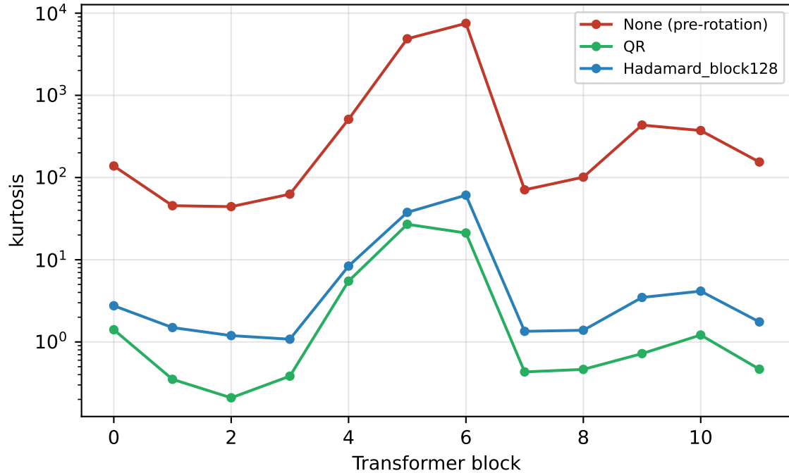
Excess kurtosis (log scale)
