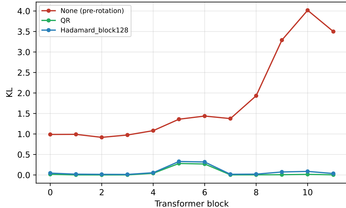
KL divergence to fitted Gaussian
