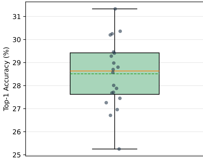
RoViT ViT-Base W4A4 mean 28.51 \pm 1.466 (n=20)
