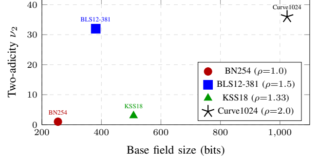
Fig. 2. Pairing-friendly curve comparison: field size vs. two-adicity. Curve1024 achieves the highest two-adicity (36) and ECDLP security (256-bit) at the cost of a larger \rho -value.
