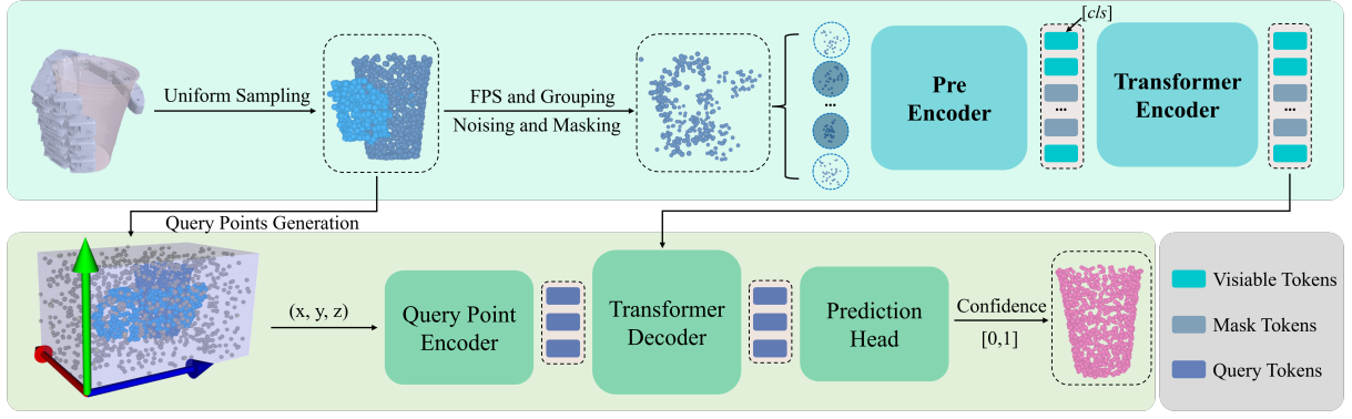
Fig. 2. Pre-Training Framework. First, noise is added to and masked from the original hand-object interaction point cloud to generate input data. Then, features are extracted using a pre-encoder and a Transformer encoder. Finally, the generated query points and a Transformer decoder are employed to accomplish the point cloud reconstruction task for the object.
