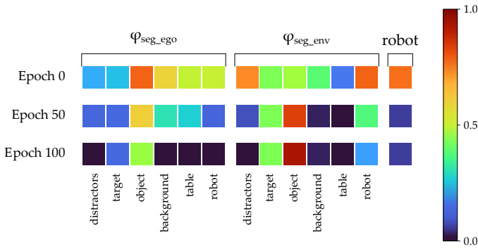
Fig. 5. Learned mask over the course of training. Our method learns a mask M \in \mathbb{R}^{n \times n} , and computes the latent state as z = Ms . Therefore, the magnitude of the i -th column of M corresponds to the i -th element of s . Here, we show how the weights of the state change as the policy training progresses. We label which components of the column relate to which information in the scene. The components with a dark blue shade have values closer to 0, indicating that the corresponding feature of the scene is removed from z . In contrast, the components with a red shade have values closer to 1, indicating that the associated feature is retained in z .
