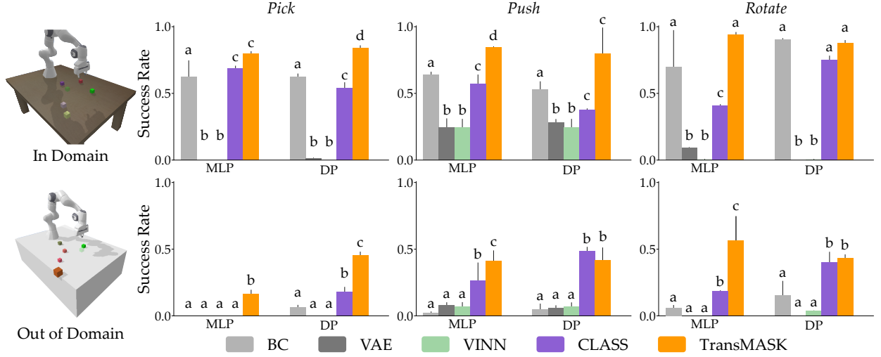
Fig. 4. Results from our simulated experiments. We perform the simulated experiments in three tasks — Pick , Push , and Rotate . The methods are trained with two different policy heads: a fully connected policy (MLP) and a diffusion policy (DP). We evaluate the methods in two scenes, denoted as In-Distribution or ID (over wooden table, top row), and Out-of-Distribution or OOD (over marble table, bottom row). All methods are trained on demonstrations collected in the ID scene, except VINN and CLASS which are trained on demonstrations from both ID and OOD scenes. We use the Compact Letter Display (CLD) algorithm [44] which assigns letters to each policy. The policies which do not share a letter have statistically significant difference in their results.
