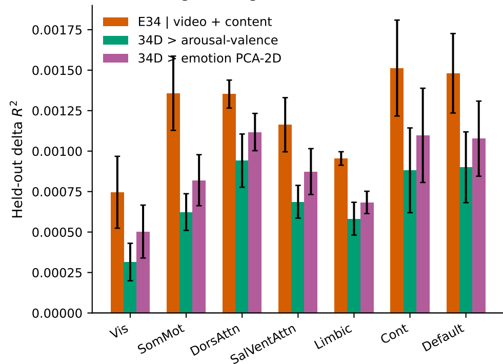
Fine-grained gain across Yeo networks
